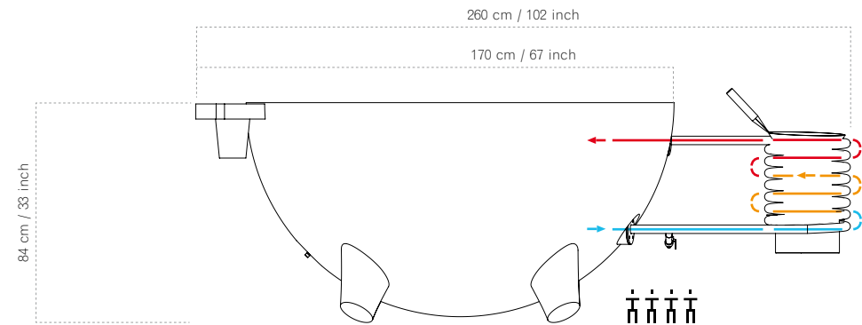
SIDE VIEW MEASUREMENTS & WATER CIRCULATION
