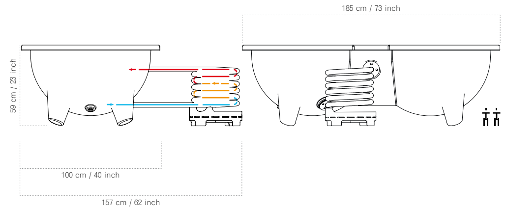
SIDE VIEW MEASUREMENTS & WATER CIRCULATION
